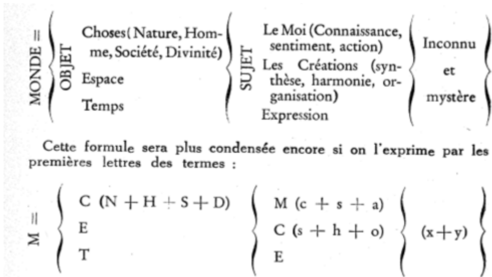
OTLET'S FORMULA
